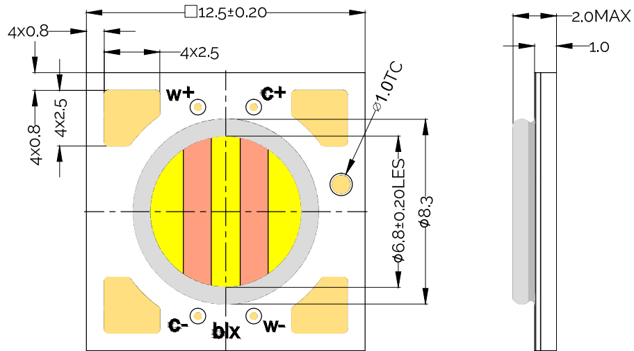
Figure 19: Mechanical Drawing Specifications
