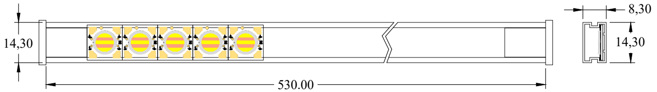
Figure 22: Vesta Series Tunable White 6mm Packaging and Labeling
